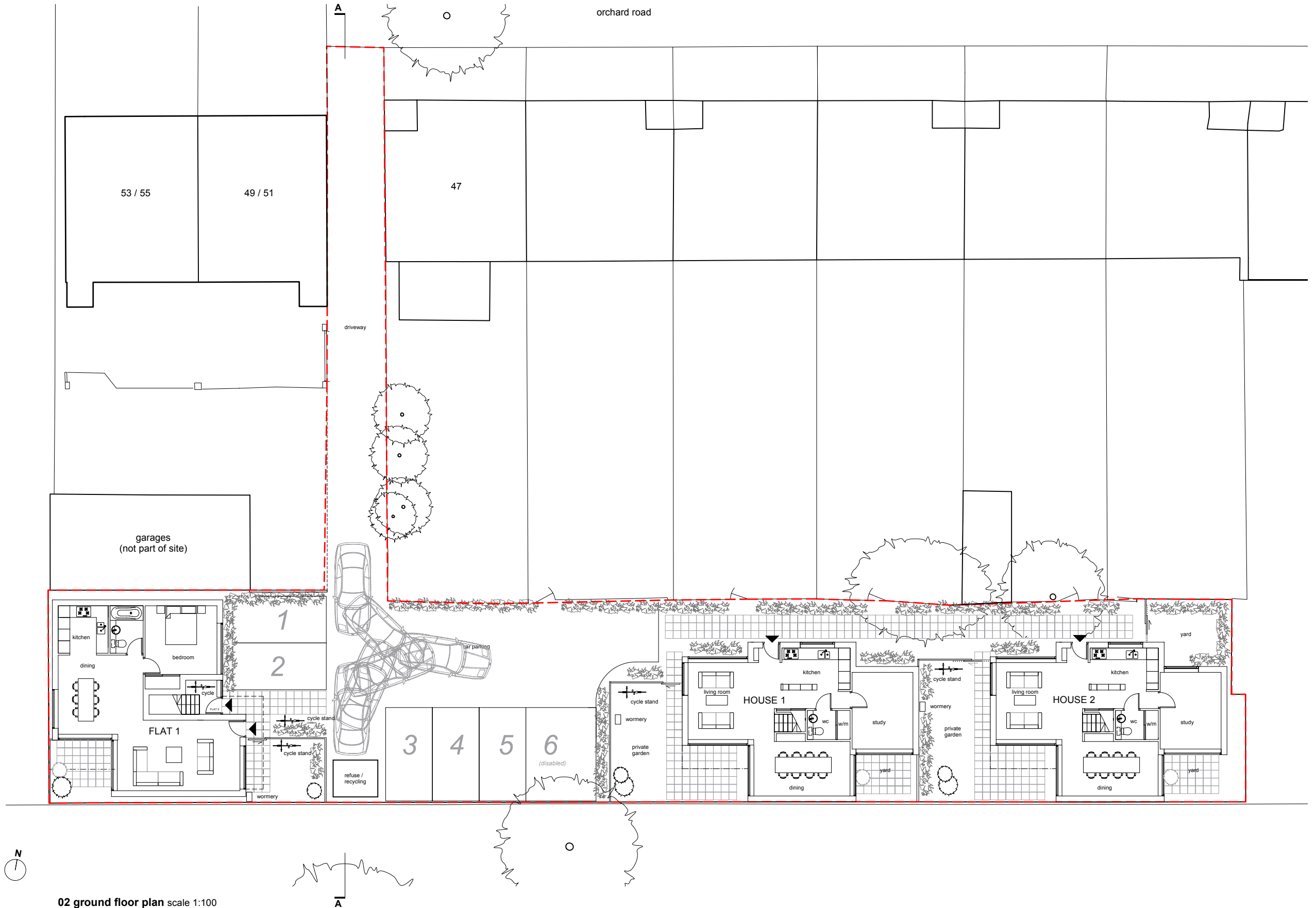
02 ground floor plan scale 1:100
